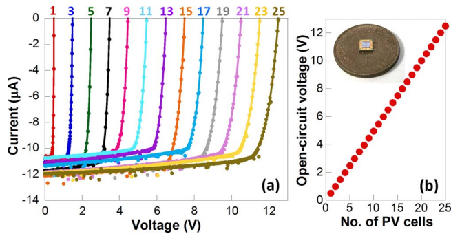
FIGURE 3. Characteristics of the CMOS PV mini-module in which PV cells are serially-connected: (a) Measured current-voltage characteristics of CMOS PV mini-module under 6 \text{ mW/mm}^2 illumination. The inset values indicate the number of PV cells to be serially connected during the measurements. (b) Measured open-circuit voltage versus the number of serially-connected PV cells.
