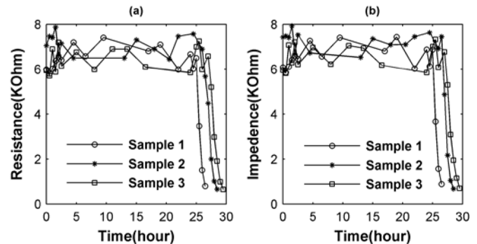
FIGURE 4. Temporal change of (a) DC resistance (with 0.1 V) and (b) AC impedance (with 0.1 V RMS , 1 kHz) of spiral thin film devices during the dissolution of glass substrate (2.2 mm thick, 14 mm diameter). This demonstrates the device performance during the stage B - D in Fig. 1.
