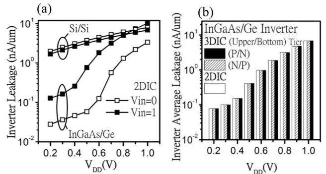
FIGURE 3. (a) Leakage comparison of 2D Si/Si and InGaAs/Ge inverters versus V_{DD} with input signal at “0” and “1”, and (b) average leakage comparison of 2D and 3D InGaAs/Ge inverters versus V_{DD} .
