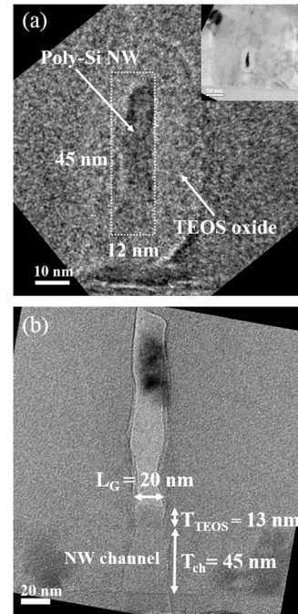
FIGURE 2. (a) Cross-sectional TEM images of poly-Si NW surrounded by gate dielectric (TEOS oxide = 13 nm) and a poly-Si gate with channel width \sim 12 nm and thickness \sim 45 nm. (b) TEM image along the channel direction showing the physical gate length is \sim 20 nm.
