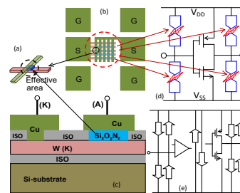
Fig. 5 Above-IC nano crossbar array ESD protection structure: (a) Single-node device, (b) 5 × 5 array, (c) X-section, (d) new on-chip ESD circuit scheme, and (e) traditional ESD protection using PN-based ESD devices.
