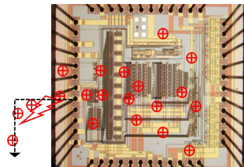
Fig. 8 Illustration of internal-oriented from-Internal-to-External ESD discharging phenomena associated with CDM ESD test standard.
