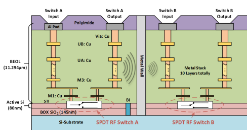
Fig. 3 X-section of in-BEOL metal wall isolation structure uses to isolate global flying crosstalk between SPDT circuits in a SOI CMOS technology.
