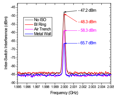
Fig. 4 Measurement comparison for SPDT circuit splits, with and without metal cage isolation, and with unfilled air trench and using standard buried isolation (BI ring), shows that the new in-BEOL metal wall structure is very efficient in EMI suppression.
