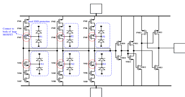
Fig. 12 The new non-pad-based internal-distributed CDM ESD protection concept was validated using a 3-stage oscillator IC implemented in a foundry 45nm SOI CMOS where a set of diode ESD devices were placed at critical internal circuit nodes for local ESD discharging internally.
