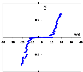
Fig. 6 ESD discharging I-V characteristics for a 5X5 array nano crossbar ESD protection structure ( 5\mu\text{m} \times 5\mu\text{m} node) by TLP measurement.
