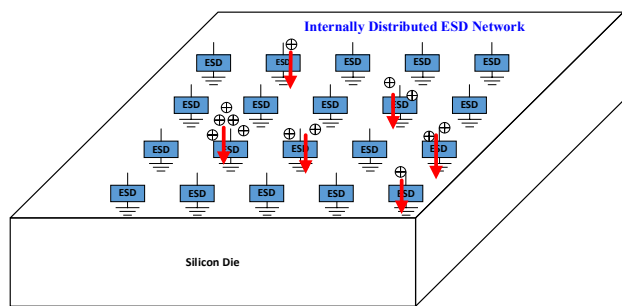
Fig. 11 Illustration of the new internal-distributed CDM ESD protection method using a non-pad-based internal ESD device mesh on a chip.
