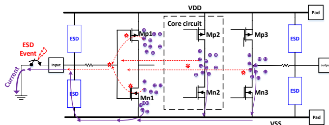
Fig. 10 Using pad-based CDM ESD protection approach cannot avoid random internal CDM ESD failures induced by internal ESD discharge current routing. (* indicates possible internal CDM ESD failure points)
