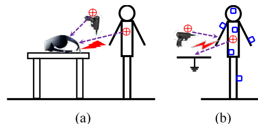
Fig. 1 ESD phenomena for (a) freestanding systems per IEC/HMM and (b) wearable electronics are very different in ESD mechanisms.
