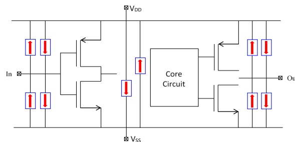
Fig. 8 Illustration of internal-oriented from-Internal-to-External ESD discharging phenomena associated with CDM ESD test standard.
