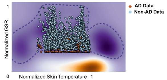
FIGURE 5. The “test” model developed with an RBF kernel distinguishes AD and non-AD data.
