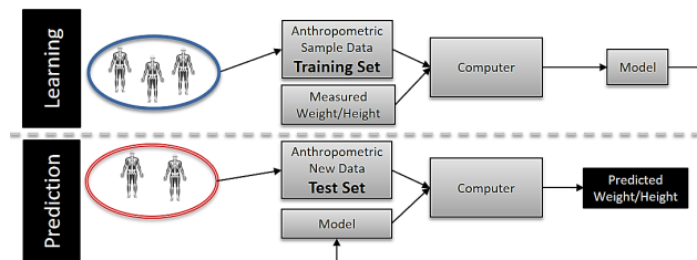
FIGURE 1. Comparison between traditional and machine learning work-flow regressions.
