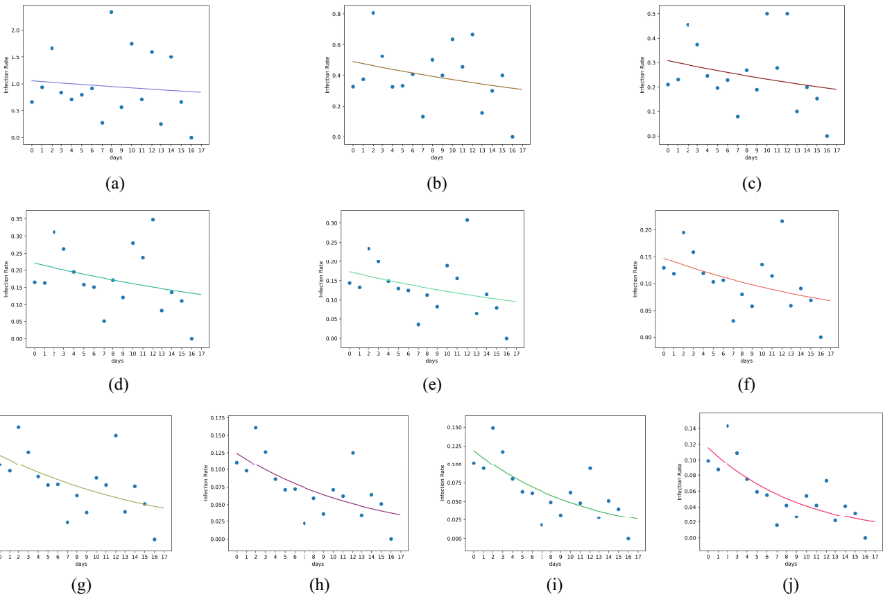
Fig. 5. Fitting curves of infection rate \beta_1 in Shanghai. (a) k = 1 . (b) k = 2 . (c) k = 3 . (d) k = 4 . (e) k = 5 . (f) k = 6 . (g) k = 7 . (h) k = 8 . (i) k = 9 . (j) k = 10 .
