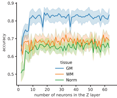
Fig. 2. Evolution of the accuracy (and its SD over the cross-validation folds) of the AD vs CTL setting when varying the number of neurons in the Z layer.
