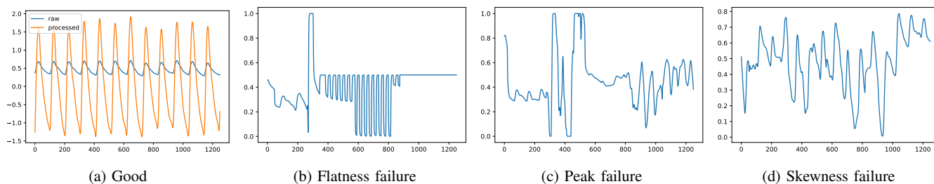
Fig. 2: Examples of PPG segments with different qualities. (a) shows a segment that passed the quality control with the raw signal shown in blue and the processed signal shown in orange. (b)-(d) are segments that failed due to different quality control criteria listed in the pre-processing steps.
