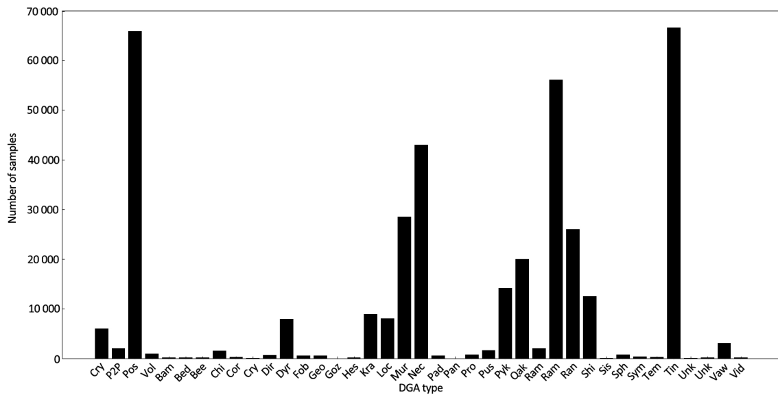
Fig. 2 Number of samples in different DGA families.
