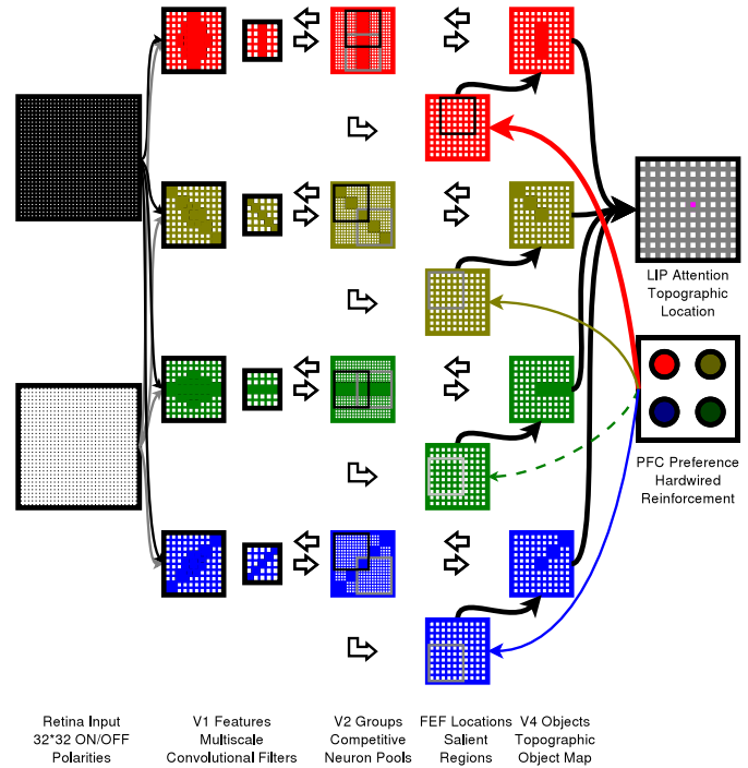
Fig. 5. Enhanced network. This shows the network as it is with all enhancements turned ON. The input retina layer is a real or simulated visual field taken either from the preprocessed robot imaging system or from a software image generator. Each of layers V1, V2, V4, and prefrontal cortex (PFC) are separated into four orientations per layer. Layer lateral intraparietal cortex (LIP) merges orientations via a WTA. Except for the input retinal layer, the PFC layer and the output LIP layer, the diagram shows one “tile” representing a particular topographic location from the retinal field; tiles extend over the entire visual field. Each of the large and small boxes in V1 represents a different scale of convolutional filter. In V2, the internal black and gray boxes represent a mapping from one of the smaller V1 filters. The black one represents the filter shown in the diagram, while gray represents another filter (not shown). Open “wide” arrows represent connections that are understood to extend over all tiles in a layer but to connect pairs of tiles at the same topographic position in each layer. Closed “narrow” arrows represent one-to-one connections between specific neurons in their associated layers with strength given by linewidth. Feedback connections project in each case so that each actual synaptic link established is bidirectional.
