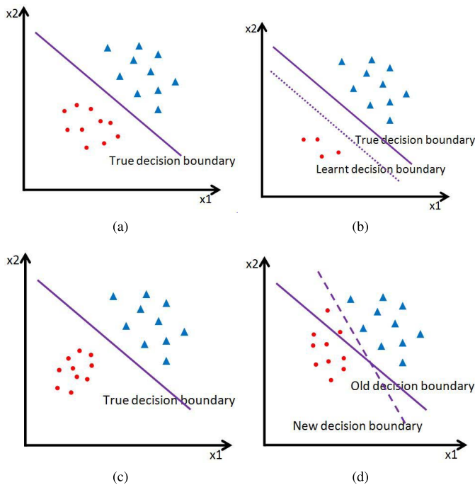
Fig. 2. Illustration of three concept drift types. (a) Original distribution. (b) P(y) drift. (c) p(x|y) drift. (d) P(y|x) drift.
