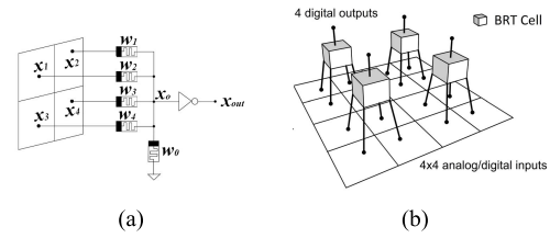
Fig. 25. (a) Modular bivalent programmable resistance MTL cell that used four-input pixel values. (b) Architectural representation of the cell arrangement for a 4 \times 4 pixels image; in this configuration, each cell uses four analog/digital inputs, has bivalued weights, and implements image dimensionality reduction [97].
