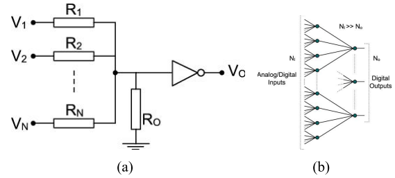
Fig. 18. Memory network cell and architecture. (a) Cell structure. (b) Network architecture (each node represents a cell) with no crossover wiring. Cells are arranged in hierarchical manner with N1 \gg N0 [88].
