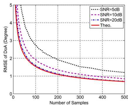
Fig. 1. Analytical and simulated RMSE of SLS DoA estimation with varying number of samples, for different SNR's with M = 9 .
