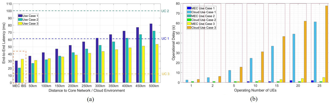
Figure 4. Evaluation of the proposed use cases in the context of MEC adaptability. (a) Simulating latency. (b) Simulating scalability.
