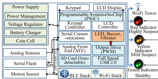
Figure 4. Architecture of proposed EasyBand.
