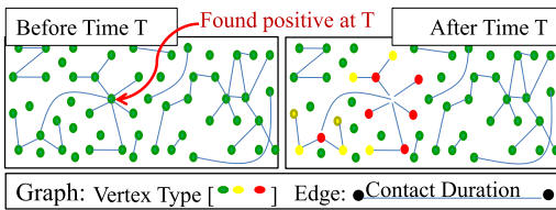
Figure 2. Contact graph before and after time T of finding a positive.
