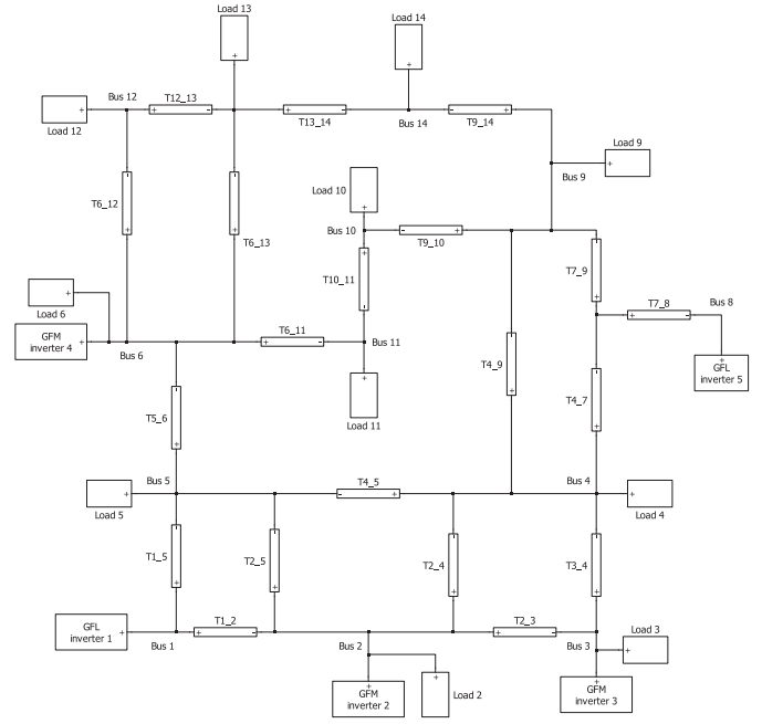
Fig. 3. The single line diagram of the modified IEEE-14 bus test system.
