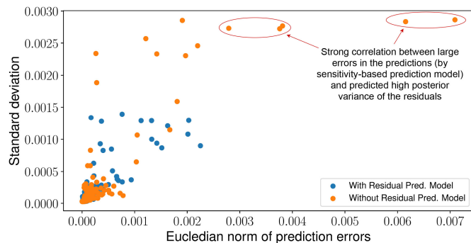
Fig. 8. Predicted standard deviation of the posterior residual distribution and prediction errors for two cases: with and without using the inferred knowledge about the residuals in secondary control.
