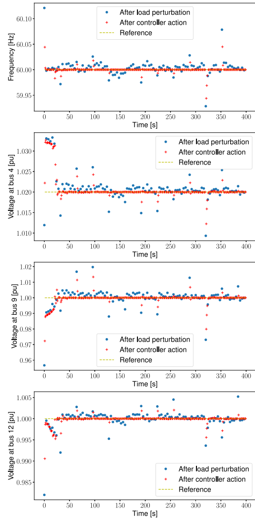
Fig. 5. Trajectories of system frequency, and voltage magnitudes at buses 4, 9, and 12.
