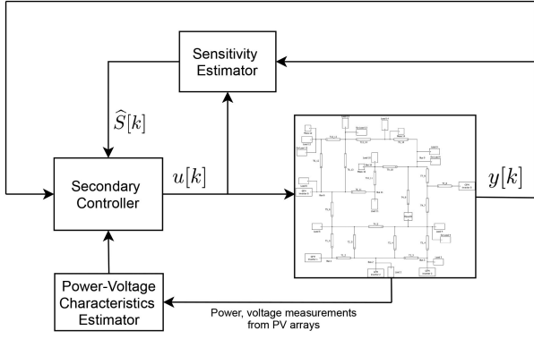
Fig. 1. Diagram of the proposed data-driven secondary controller.
