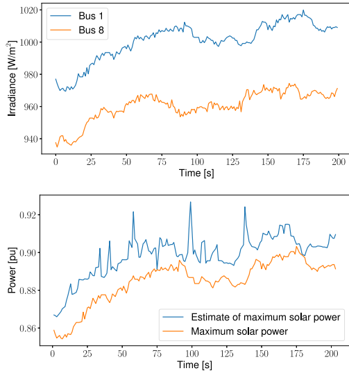
Fig. 4. Solar irradiance profile at buses 1 and 8, maximum available solar power at bus 1 and its estimate.
