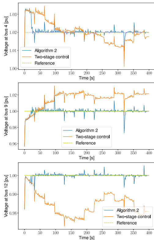
Fig. 7. Trajectories of the voltage magnitudes at buses 4, 9, and 12 for Algorithm 2 and two-stage voltage control approach [25].
