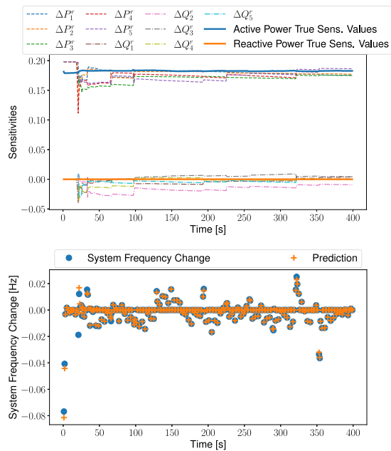
Fig. 6. Evolution of the estimated sensitivities corresponding to system frequency, and the actual sensitivity values, and predictions of the frequency changes.
