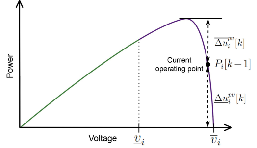
Fig. 2. Illustration of the relaxation of the power-voltage characteristic (34e) subject to an interval voltage constraint (34f) to the interval power constraint based on the incremental capacities of a PV array with respect to the current operating point.
