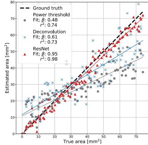
Fig. 5. In silico area estimation results. The plots show area estimates using ResNet, DC, and power thresholding on a test dataset simulated similar to the training dataset. Linear regression slopes and coefficients of determination are denoted by \beta and r^2 . Ground truth refers to the areas of the ground-truth masks.
