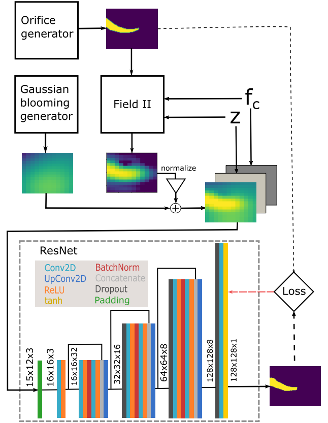
Fig. 2. Schematic representation of the network training. Binary maps representing regurgitant orifices are procedurally generated. Their power-Doppler responses are simulated using Field-II, and the Gaussian blooming artifacts are superimposed to the normalized images. The resulting images, along with the depth z and frequency f_c parameters, are used to train a CNN (ResNet) to perform segmentation from the power-Doppler images.
