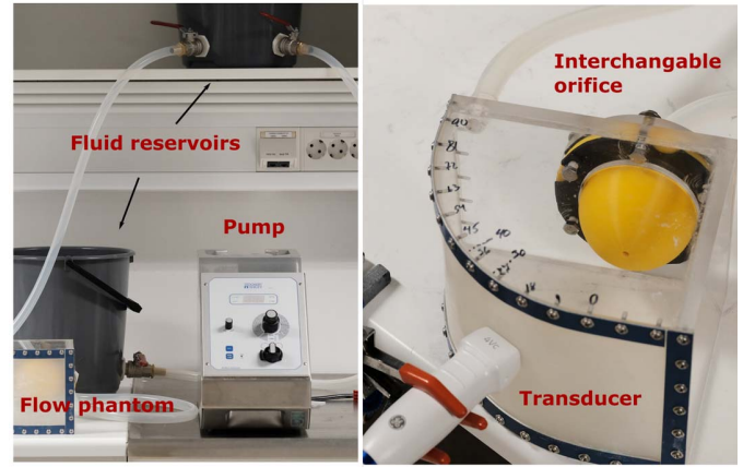
Fig. 3. Experimental setup. (Left) Overview and (right) flow phantom closeup.
