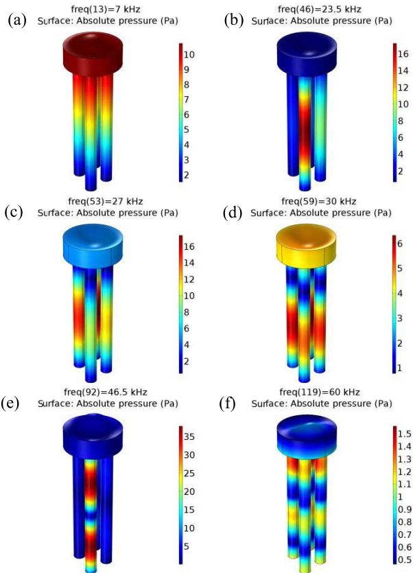
Fig. 5. The pressure (different resonances) in the pipes and cavity and the vibration of the thin plate when frequency is (a) 7kHz, (b) 23.5 kHz, (c) 27 kHz, (d) 30 kHz, (e) 46.5 kHz, and (f) 60 kHz for the 4 pipes device (III), with (a)–(f) corresponding to the frequency in Fig. 6.
