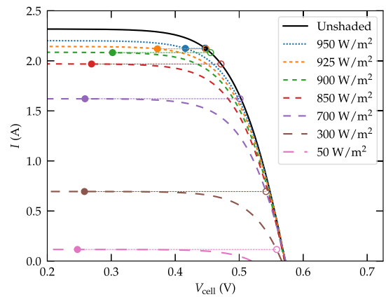
Fig. 8. I - V curves of the unshaded cells (black) and a single shaded cell subjected to varying levels of illumination. The black dot indicates the MPP when no cells are shaded; the filled dots show the operating point of the shaded cell, while the open dots on the unshaded I - V curve show the corresponding operating point of the unshaded cells. The model uses the measured value R_{\text{shunt}} = 2268 \Omega to characterize \tilde{g} at short circuit.
