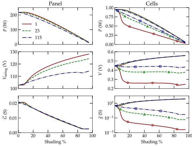
Fig. 9. Response of a 230-cell string under 1-sun illumination when 1 (red line), 23 (green dashed line), or 115 (blue dash-dot line) cells are shaded by the percentage indicated on the horizontal axis. The left column describes the full panel; the right column shows properties of individual cells, with the unshaded cells in the upper curves and the shaded cells ( \circ , \triangle , \square ) in the lower curves.
