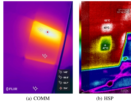
Fig. 7. (a) Thermal image of the shaded cell on a COMM panel documenting a hotspot of 154°C. (b) Thermal image (Seek CompactPro) of a HSP panel showing a temperature of 47°C on the shaded portion (green) of the shaded cell. A temperature of 53°C is recorded on the illuminated portion (upper, white) of the shaded cell, and a temperature of 52°C is recorded on an unshaded neighboring cell located just above the shaded cell.
