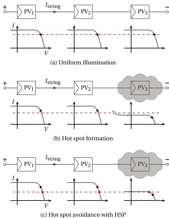
Fig. 4. (a) Three identical, fully and uniformly illuminated PV cells in a string are operating at the same point on their common I - V curves. (b) PV_3 is now partially shaded, reducing its photocurrent. A conventional MPPT controller sends the PV_3 operating point into reverse bias (open red dot). PV_1 and PV_2 shift to higher voltage to match their current to that of PV_3 . (c) Kernahan's controller sets the operating current to just below I_{sc} of the shaded cell, avoiding a hot spot. All Panels: Dark dots are the initial operating points and red dots are the final operating points due to the shading of PV_3 .
