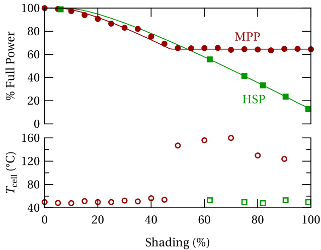
Fig. 6. Top panel: Output power as a function of percent shading of a single cell in a COMM panel under MPPT control (filled red circles) and in an HSP panel (filled green squares). In both cases, the power output with a shaded cell is normalized by the full power with the shade removed. The red curve shows a simulation of the expected behavior of the COMM panel with a lossless controller. The green curve is a simulation of expected behavior of the HSP panel as described in detail in Section IV. Bottom panel: The temperatures of the shaded cells in the COMM panel (open red circles) and in the HSP panel (open green squares) versus shading of a single cell. The shaded COMM cell remains roughly 25°C above ambient as shading increases and current decreases until the shading exceeds 48%. At this point, the MPPT controller raises the current, which activates the bypass diode of the string with the shaded cell. The temperature of the shaded cell then rises as high as 160°C for 70% shading. The shaded HSP cell (open green squares) shows no temperature rise for this high level of shading, but shows output power that decreases linearly with shading, albeit with an offset we attribute to light leaking through the back of the panel.
