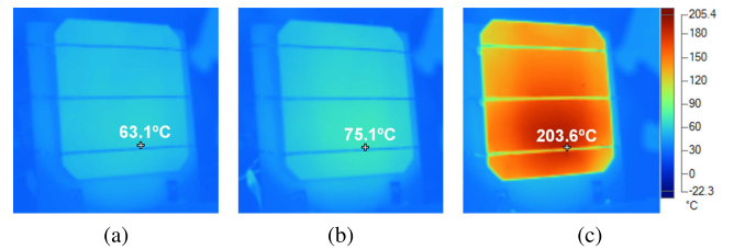
Fig. 3. Thermal images of a solar cell under three different conditions: (a) the cell near maximum power generation at 63^\circ\text{C} with cell voltage = 0.38 V and 1.0-sun-ETC illumination, (b) the cell in short circuit at 75^\circ\text{C} and 1.0-sun-ETC illumination, and (c) the cell under reverse bias at 204^\circ\text{C} with cell voltage = -12 V and 0.8-sun-ETC illumination. All thermal images use the same color coding displayed on the right side of the figure.
