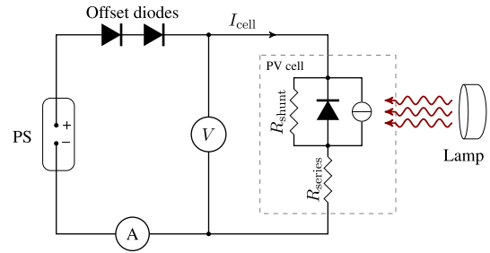
Fig. 2. Experimental setup for measuring the I - V curve of a single PV cell, and subsequently observing the temperature rise and damage sustained when forced into reverse bias. PS = HP6267B power supply; V and A are two Tektronix DM2510 G multimeters for measuring the cell voltage and current, respectively; the offset diodes are Diodes, Inc., SBR20A200CT; and the lamp is an ETC Source 4 Ellipsoidal 750W 36° 436 spotlight.
