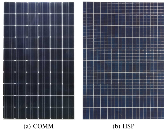
Fig. 5. Two types of PV panels were tested: (a) a popular commercial panel (COMM) with a 6 \times 10 array of standard-size cells, and (b) a HSP panel with a 23 \times 10 array of quarter-width cells.
