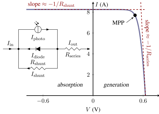
Fig. 1. Equivalent dc circuit model for a PV cell (left inset), and a room-temperature I - V curve for the Everbright grade A full-size (156 mm \times 156 mm) PV cell.
