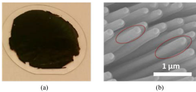
Fig. 9. (a) A peeled GaAs NW membrane, after transfer to a 2" glass carrier. (b) We found that NWs on these membranes are tilted. Subsequent dry etching damages the side-wall of the emitter and pn-junction, causing shunt leakage in many cells. Specifically, the oxide near the top of the NWs is fully etched (see circles). We can avoid this issue by combining the NWs and cell integration concepts from concept II with the membrane procedure of concept III .
