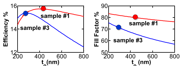
Fig. 3. (a) Efficiency versus absorber thickness for samples #1 and #3. (b) Fill factor versus absorber thickness for samples #1 and #3.
