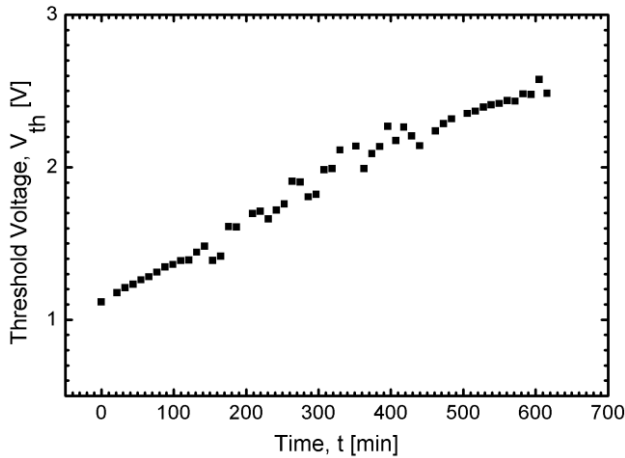
Fig. 5. Variation of the threshold voltage of the proposed E-mode MOS-HEMT employing 20 nm thick SiO 2 gate dielectric with stress time.
