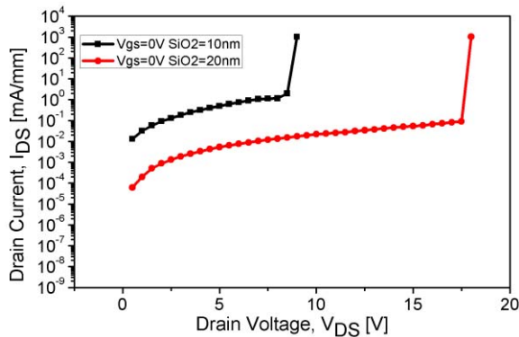
Fig. 4. Breakdown characteristics of E-mode 6\mu\text{m} \times 100\mu\text{m} AlGaIn/GaN MOS-HEMTs with 10 nm and 20 nm thick SiO 2 gate dielectrics.
