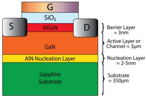
Fig. 1. Cross-section of the proposed E-mode AlGaN/GaN device.
