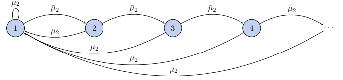
Fig. 2. The DTMC that models the AoI evolution.
