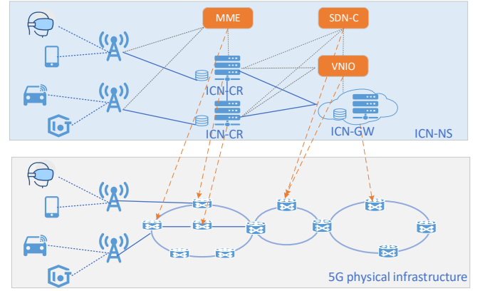
Fig. 2. An illustrative example: A 5G ICN NS.
