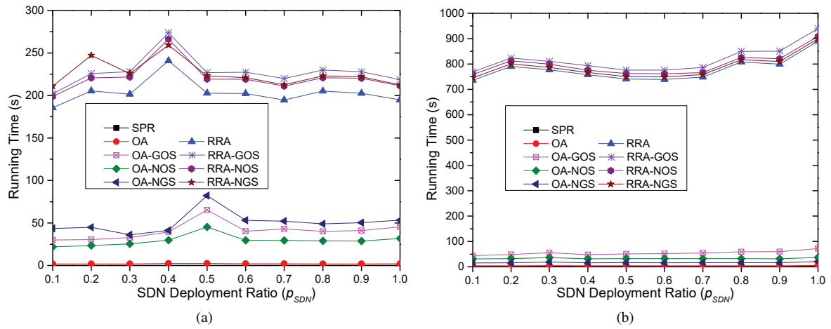
Fig. 6. The running times of the algorithms in real ISP topologies when the SDN deployment ratio p_{SDN} varies: (a) Garr and (b) VtWavenet2011.
