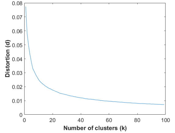
Fig. 3. The relationship between distortion values and number of clusters as obtained using Elbow
