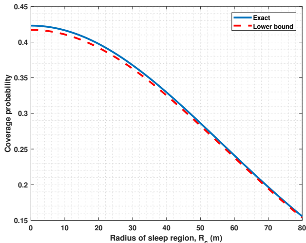
Fig. 7. Comparison of the exact coverage probability of the typical femto user and its lower bound with \lambda_f = 10\lambda_m ( \lambda_m = 4.973 \times 10^{-5} ), \sigma^2 = 5 \times 10^{-4} ( \text{SNR}_f = 23 dB).
