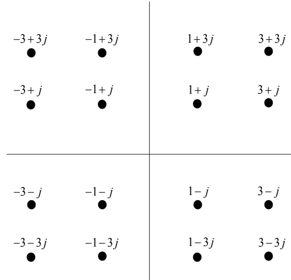
Fig. 1. 16-QAM constellation.
