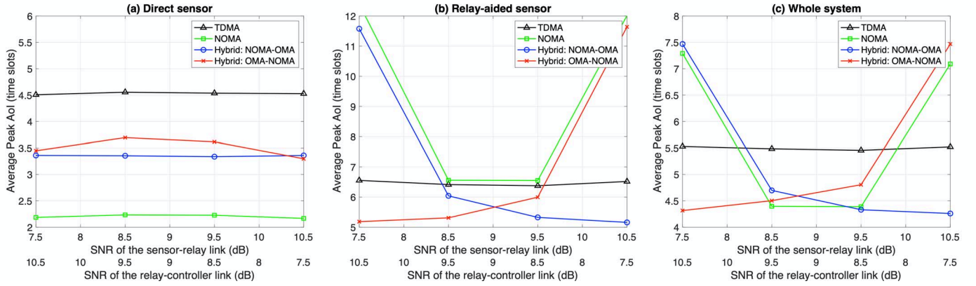
Fig. 7. SDR experimental results for the average peak AoI of (a) the direct sensor, (b) the relay-aided sensor, and (c) the whole system under different CDRT schemes with the SNR-imbalanced scenario, where the SNR from the direct sensor to the controller and the relay in (a)–(c) are fixed at 9.5 dB.
