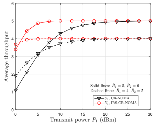
Fig. 6. Average throughput comparison for U_1 .
