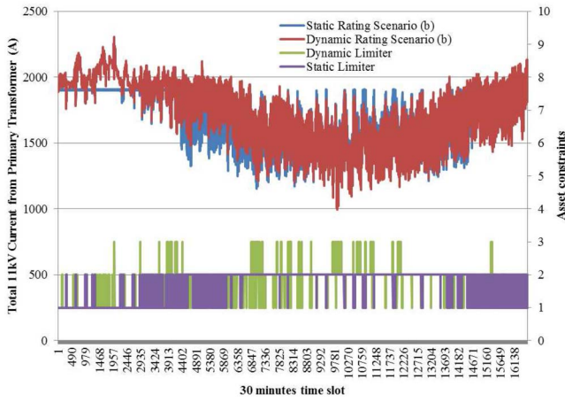
Fig. 14. DNR of the circuit under scenario (b) (OFAF cooling, un-ducted cable, wind angle 0°).
