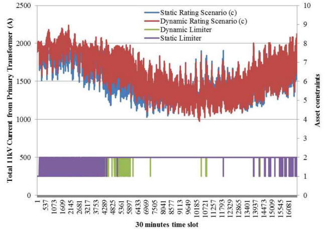
Fig. 16. DNR of the circuit under scenario (c) (OFAF cooling, ducted cable, wind angle 45°).
