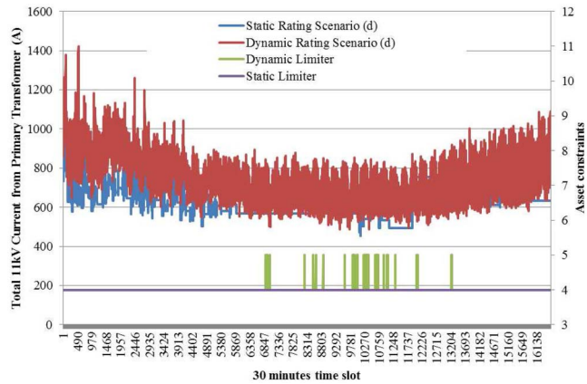
Fig. 17. DNR of the circuit under scenario (d) (OFAF cooling, ducted cable, wind angle 45° with distribution transformers).
