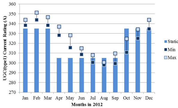
Fig. 11. DAR of the underground cable (UGC) (type 1).
