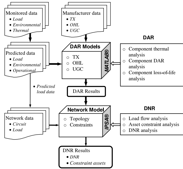
Fig. 3. Overview of the proposed DNR process.
