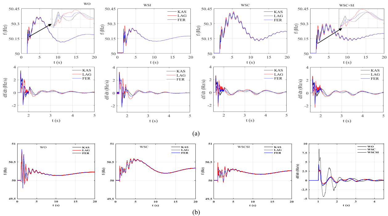
Fig. 10. System frequency and ROCOF during a three-phase short-circuit fault with WO, WSI, WSC, and WSC+SI. (a) Exporting HVDC link to Norway. (b) Importing HVDC link from Norway.
