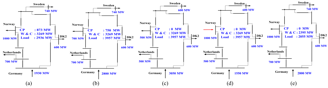
Fig. 6. Case-study scenarios (CP: central production, W & C: wind and coastal production). (a) Base case. (b) HLHW with 3 SGs. (c) HLHW no SGs, exporting to Norway. (d) HLHW no SGs, importing from Norway. (e) LWLL.
