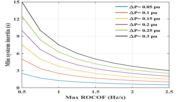
Fig. 2. The dependence of system inertia on maximum ROCOF and disturbance size.
