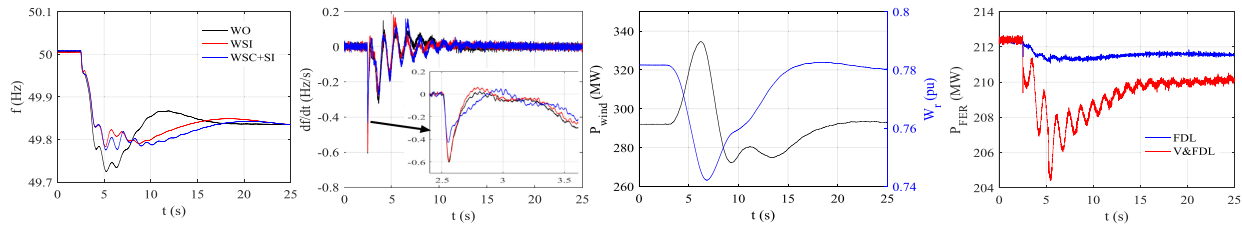
Fig. 11. System responses during a disturbance of LWLL.
