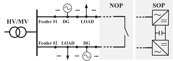
Fig. 1. Schematic of SOP installation.
