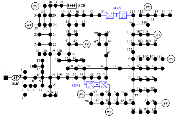
Fig. 13. Structure of the modified IEEE 123-node system.
