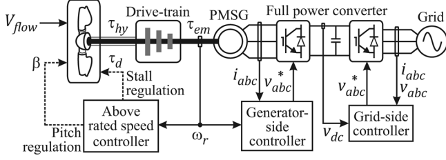
Fig. 1. TST configuration based on a PMSG and an FPC.
