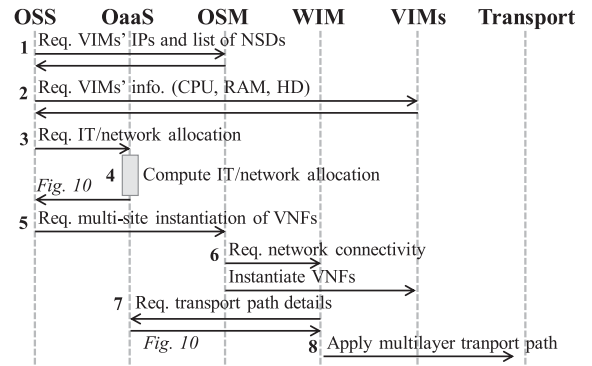
Fig. 8. Simplified schema of the workflow.
