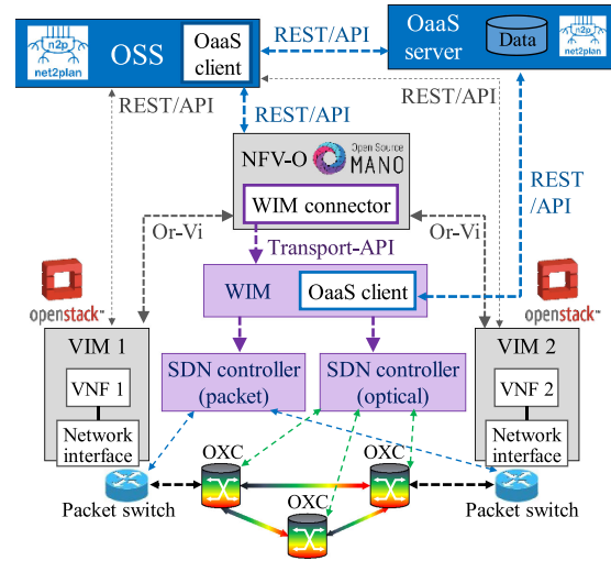
Fig. 7. Functional Architecture
