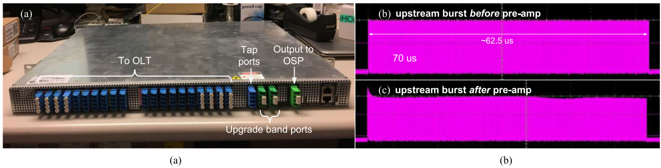
Fig. 4. (a) Photo of the FE; (b) Upstream time-domain waveform before pre-amplifier; (c) Upstream time-domain waveform after pre-amplifier.
