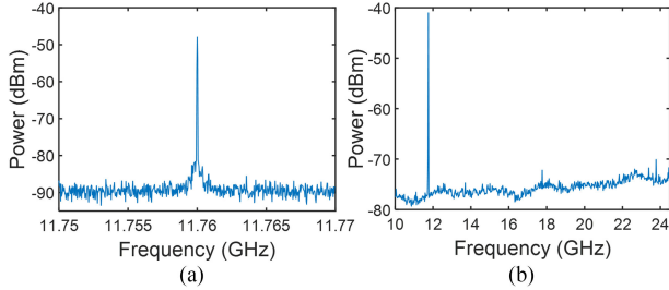
Fig. 9. Electrical spectra of the THz carrier after down-conversion to the IF frequency for (a) 240 GHz (RBW = 20 KHz, and VBW = 3 KHz), and (b) 246 GHz when it is tuned by 6 GHz electrical LO (RBW = 10 MHz, and VBW = 1 MHz).
