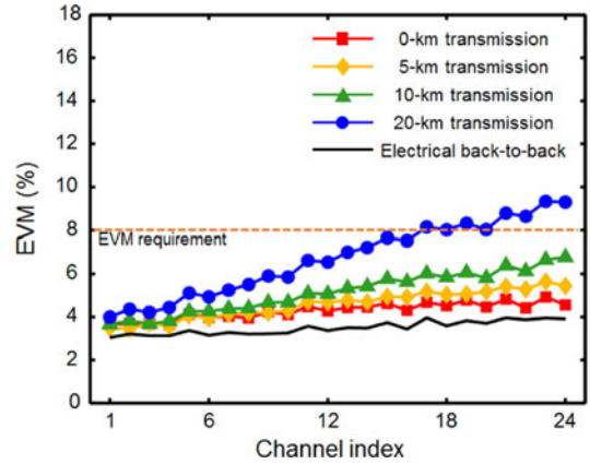
Fig. 7. EVM performances of all 24 channels measured at various transmission distances in the RoF link implemented by using 1.55- \mu\text{m} DML. The RF power per channel was set to be -13.8 dBm.
