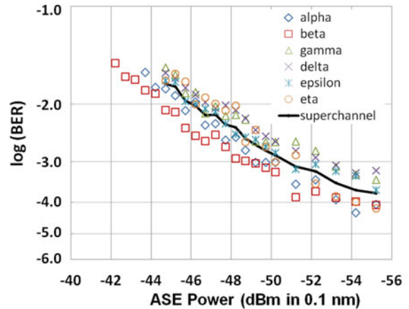
Fig. 10. Subchannel and superchannel BER as a function of added ASE loading power, for f = 191.5 THz for the Express path.
