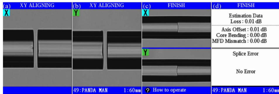
Fig. 2. Images of the PM fibers spliced with rotation of their birefringence axes by 90^\circ relative to each other inside the ring fiber cavity (as marked by a cross in Fig. 1) before [(a) and (b)] and after splicing [(c) and (d)].
