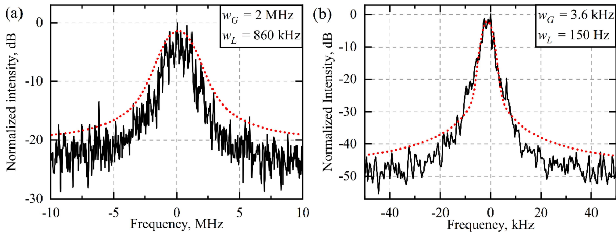
Fig. 6. Delayed self-heterodyne spectra of the free-running DFB laser (a) and the DFB laser stabilized to operate in the self-injection locking regime (b). The measured spectra (black) and their fitting Voigt profiles (red dotted line) with the Gaussian ( w_G ) and Lorentzian ( w_L ) linewidths (FWHM) used as the fitting parameters.
