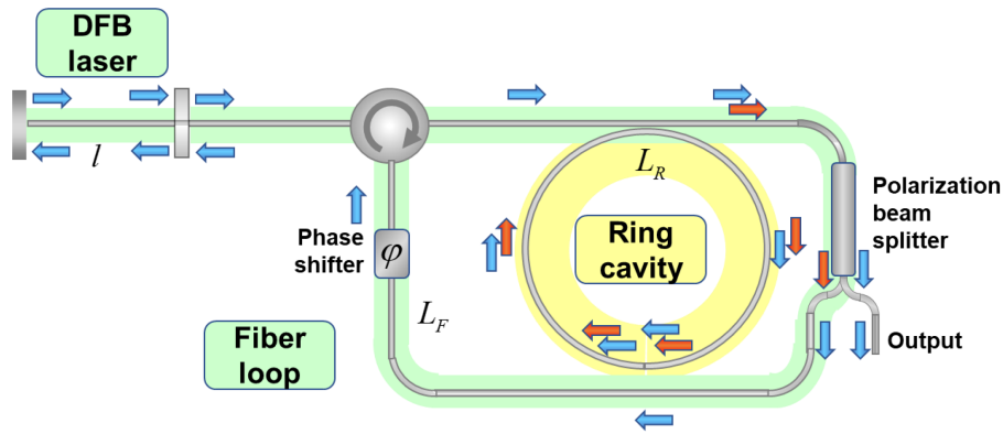
Fig. 3. Illustration to the self-injection locking laser operation. Green background shows the coupled cavity comprising the DFB laser and feedback loop possessing the resonance at \nu_{LD+FD} ; yellow background marks the ring cavity with the resonance at \nu_R . Arrows show the polarization states along the fast (red) and slow (blue) axes.
