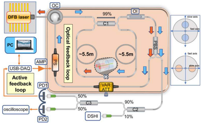
Fig. 1. Schematic illustration of the experimental configuration; OC – optical circulator, C1 – optical PM fiber coupler (both axes working), OI – optical isolator, PBS – polarizing beam splitter, VAR ATT – variable attenuator (0 – 60 dB), PS – phase shifter, C2 and C3 – non-PM single-mode fiber couplers, PD1 and PD2 – photodetectors, USB-DAQ – microcontroller, AMP – electric amplifier, DSHI – delayed self-heterodyne interferometer. The highlighted area bounded by the dashed line indicates the thermal stabilization box. On the right is shown the orientation of the fiber birefringence axes on either side of the splice.
