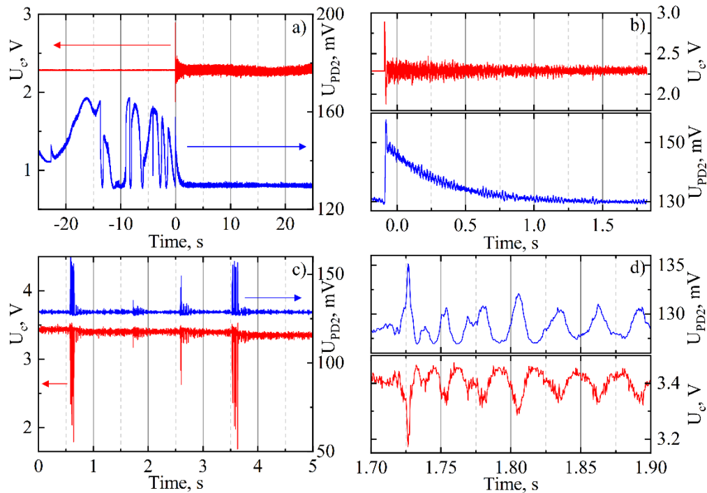
Fig. 4. Oscilloscope traces of the laser output power (the error signal produced by the photodetector) and control voltage applied to the phase shifter before ( T < 0 s) and after ( T > 0 s) the optoelectronic feedback activation.
