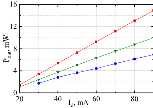
Fig. 5. Power characteristics of the free-running DFB laser (red line), the laser configuration with open ring cavity (green line) and the laser configuration stabilized to operate in the self-injection locking regime (blue line).
