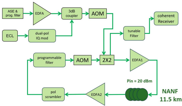
Fig. 14. Schematic of the NANF recirculating loop experiment [128].
