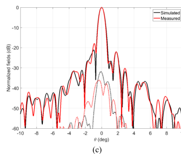
Fig. 5. Illustration of 1-m offset-fed deployable mesh reflector antenna. (a) An artist on-orbit rendition [18]. (b) Prototype antenna pattern test with gravity offload fixture at JPL near-field measurement facility. (c) A representative E-plane far-field pattern comparison between the measured and simulation results at 35.75 GHz.
