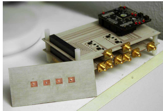
Fig. 17. Null-scanning retro-directive array antenna for CubeSat [52].
