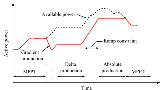
Fig. 19. Different active power control functions for the DPGS to ensure grid frequency stability [61], [62].
