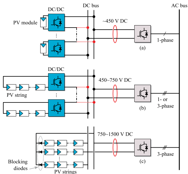
Fig. 11. Connecting PVs to the ac grid (dc bus connections can be in series or in parallel): (a) module PV inverter for low-power applications; (b) string inverter for medium-power applications; and (c) central inverters for commercial or utility-scale systems. DC–DC converters for the string inverter are optional. For high-voltage PV systems (e.g., 750–1500-V dc), transformers are required.
