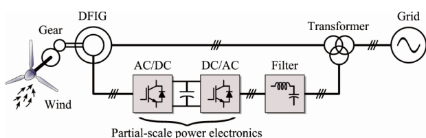
Fig. 6. Wind-turbine DPGS based on the DFIG technology with partial-scale power electronics.
