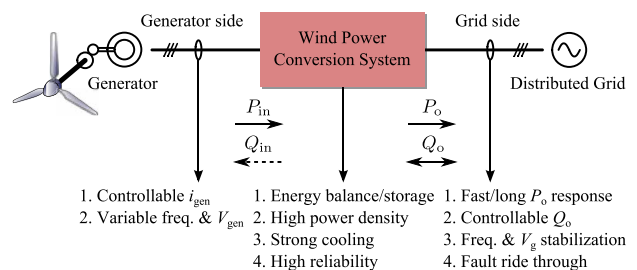
Fig. 5. Demands for the wind-turbine power-system-based DPGS, where P_{in} and Q_{in} are the active and reactive power exchanges between the generator and the power electronic converter, respectively, and P_o and Q_o are the active and reactive power exchanges between the power converter and the grid, respectively.
