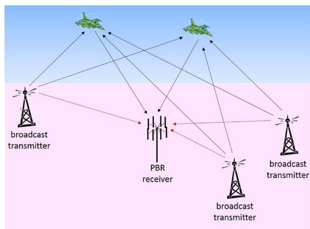
Fig. 9. Passive bistatic radar.
