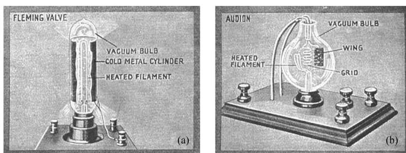
Fig. 7. (a) Fleming valve, patented in 1904 in its commercial version [56]. Operation is based on thermionic emission of electrons from the heated filament, which were attracted only to a positively charged anode. (b) “Audion” detector (triode) invented in 1907 [56]. A grid is disposed between the filament and the plate to control the charge electron displacement. (Source: http://earlyradiohistory.us/ )
