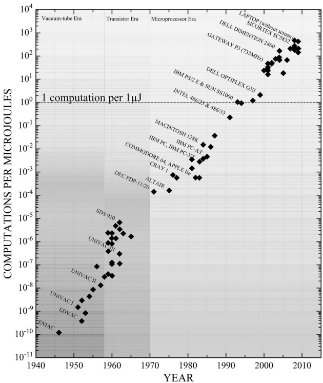
Fig. 3. Number of computations per micro-Joules averaged over an hour. A micro-Joule is the sum of 1-μW power during 1 s, or 100 nW during 10 s. (Data from [51].)
