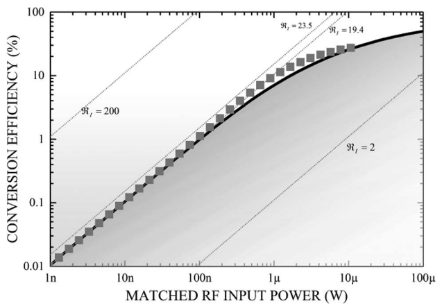
Fig. 28. Conversion efficiency in a rectifying circuit based on the SMS7630 diode under lossless matched condition. Data obtained from the low power analysis (15) are plotted in a gray short dotted line. A more complicated version of (15) taking into account the deviation from square-law operation \Delta and self-biasing V_b is plotted in gray boxes. Those data are compared to a SPICE circuit simulation under the same conditions in black solid line. Frequency is 2.45 GHz and output load is 1 k \Omega .
