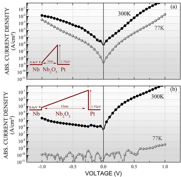
Fig. 21. Current density versus voltage characteristics of two 80-μm × 80-μm MIM diodes having (a) 5-nm and (b) 15-nm insulator thickness (also shown in Fig. 20), measured at 77 and 300 K. Insets are the trapezoidal representation of the barrier. Data from [97].
