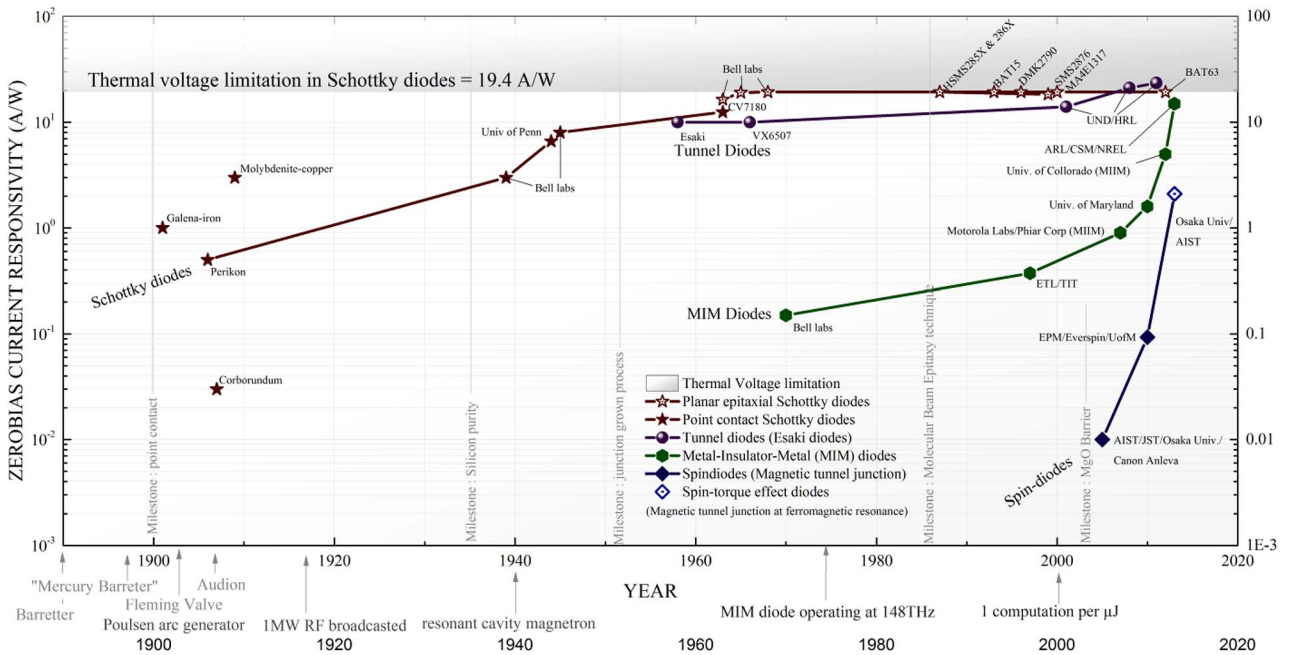
Fig. 5. Evolution of the rectification capabilities of different diode technologies over the years.
