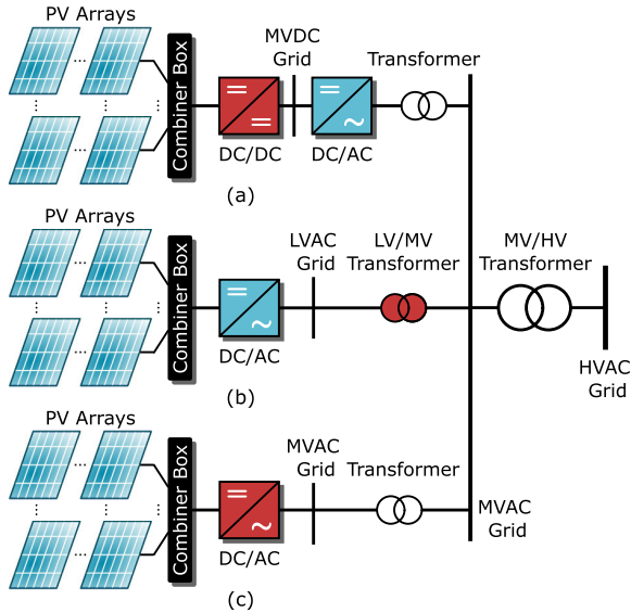
Fig. 12. Typical configurations of large-scale PV power generation systems connected to MVac grids: (a) double-stage via a boosting dc/dc converter, (b) single-stage using a boosting transformer, and (c) single-stage through a step-up inverter. Here, cascaded structures can also be used. The red dc/ac in Fig. 12(c) means that the inverter has boosting capability.
