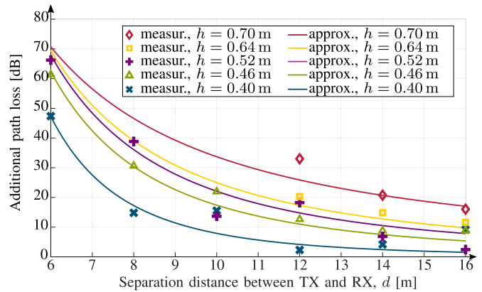
Fig. 9. Measured and modeled loss for under-vehicle propagation.
