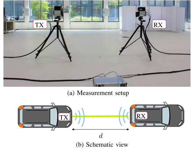
Fig. 4. Setup for the LoS propagation.
