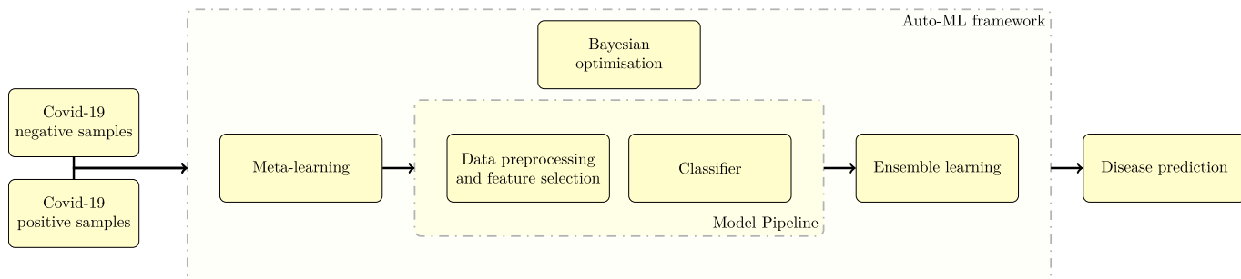
Fig. 8. Flowchart outlining the model selection process with Auto-ML [37].
