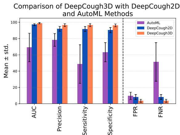
(a) Comparison of DeepCough 3D and 2D Classifiers with an Auto-ML ensemble of shallow machine learning methods [37] combined.
